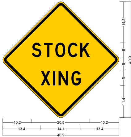
30W11-50; 30.0" across sides 1.9" Radius, 0.8" Border, 0.5" Indent, Black on Yellow; "STOCK", D; "XING", D; Table of letter and object lefts S T O C K 10.2 14.5 18.5 22.9 27.2 X I N G 13.4 17.7 19.6 24.1
